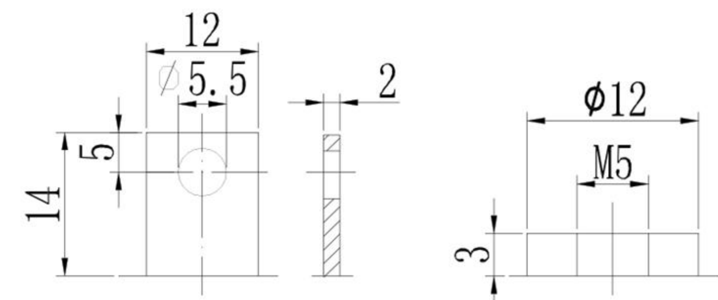
Terminal T3
