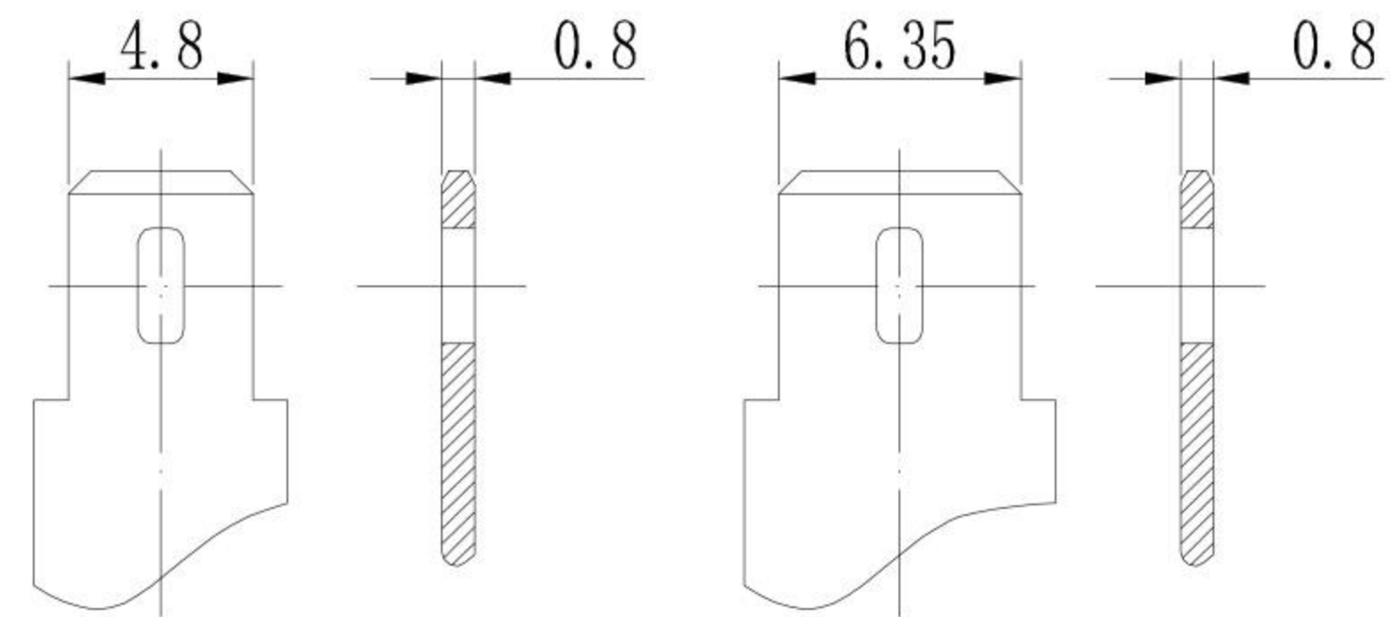
Terminal T1
